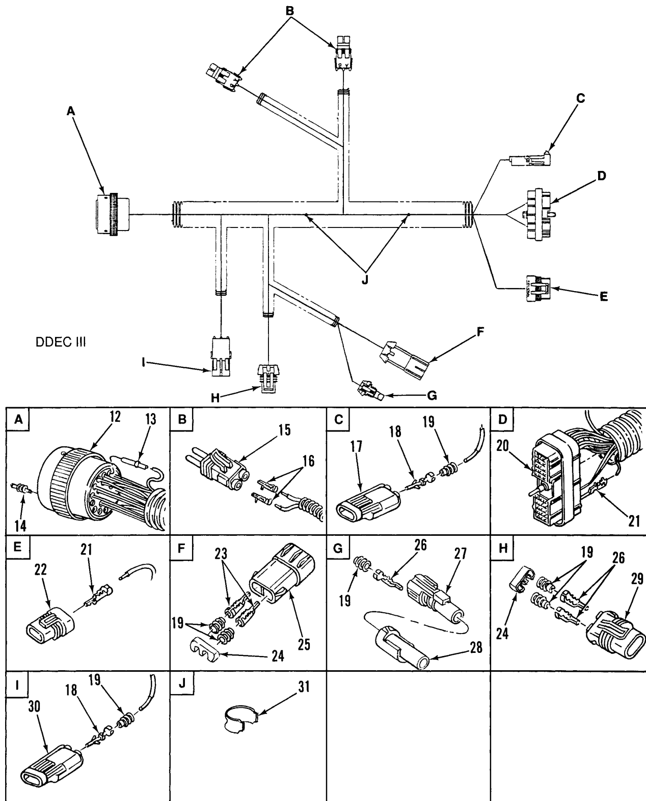
Figure 71. Engine DDEC Wiring Harness (Sheet 2 of 2)
