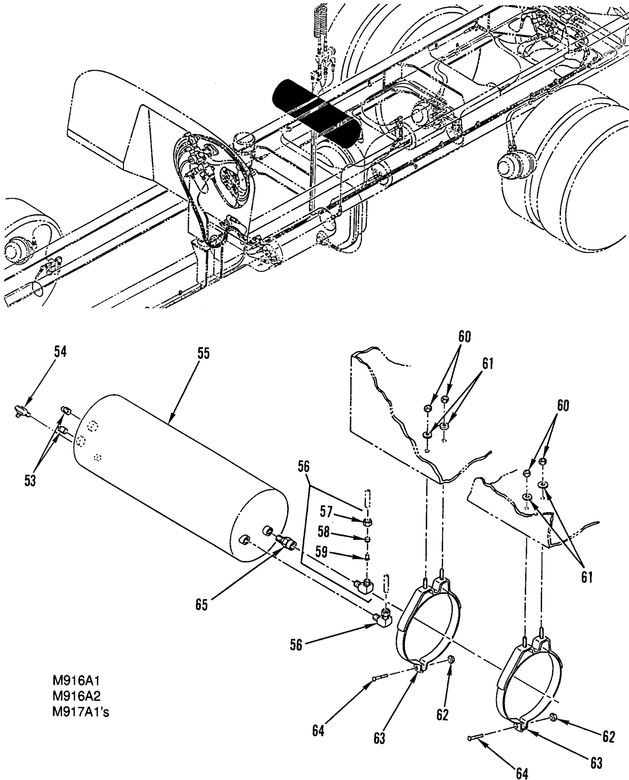
Figure 208. Air System Valves, Tanks, Lines, and Fittings, Part 10 (Sheet 2 of 2)
