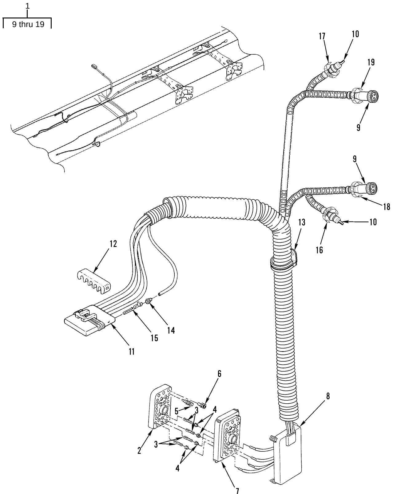
Figure 126. ABS Harness, Front (M916A2, M917A1's) (Sheet 2 of 2)
