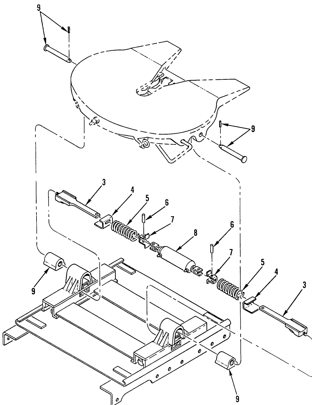
Figure 253. Slider Bracket and Plate (M915A2)
