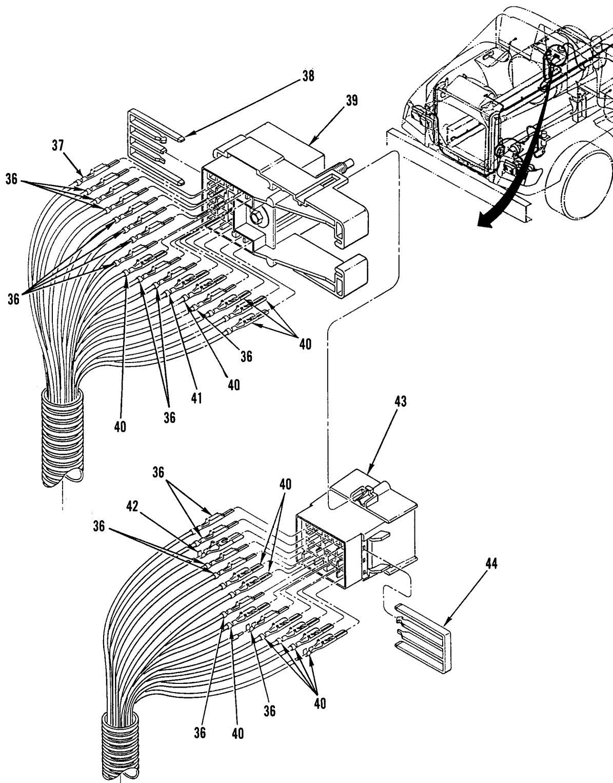
Figure 113. Chassis Wiring Harness (Sheet 3 of 3)
