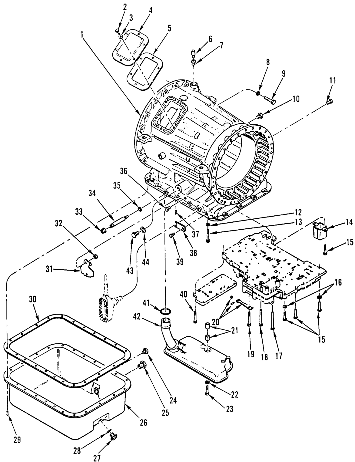
Figure 154. Transmission Housing, Oil Filter, and Oil Pan
