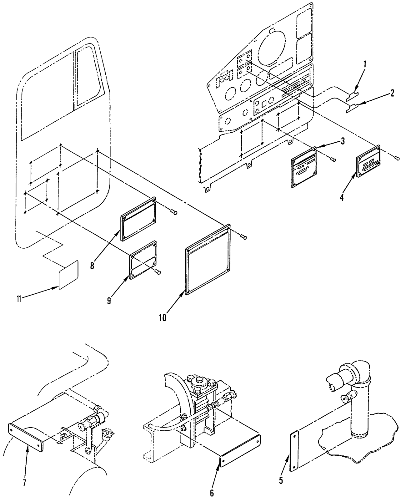
Figure 318. Data Plates
