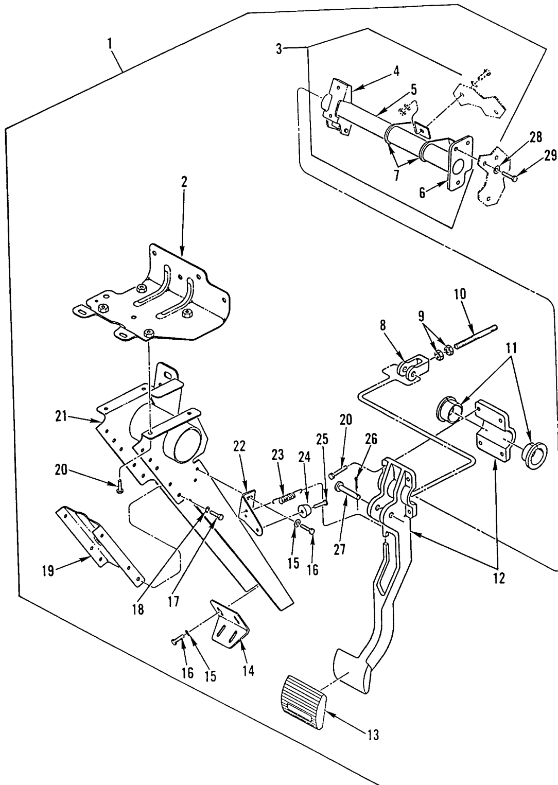
Figure 191. Hanging Brake Assembly
