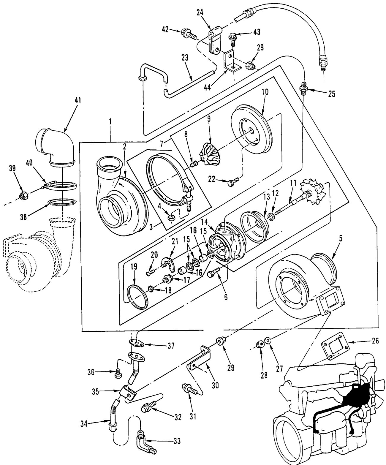
Figure 36. Turbocharger Assembly
