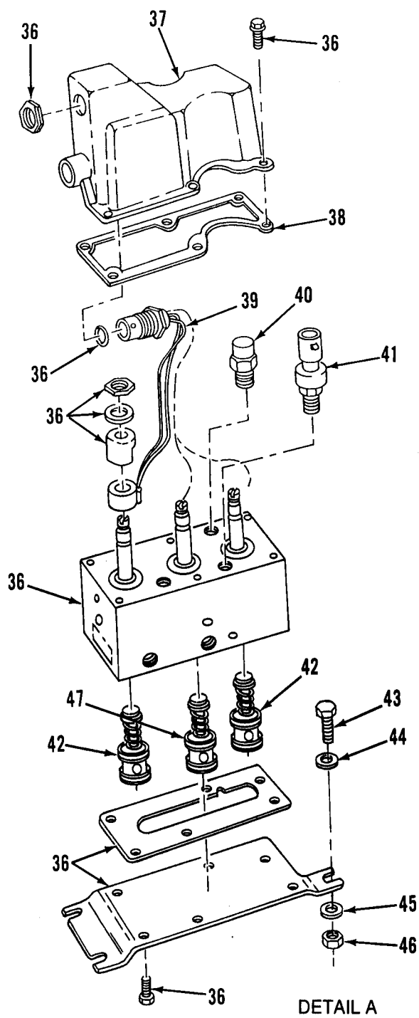
Figure 222. CTIS Lines, PCU, and Wheel Valve Assemblies (M917A1's) (Sheet 2 of 3)
