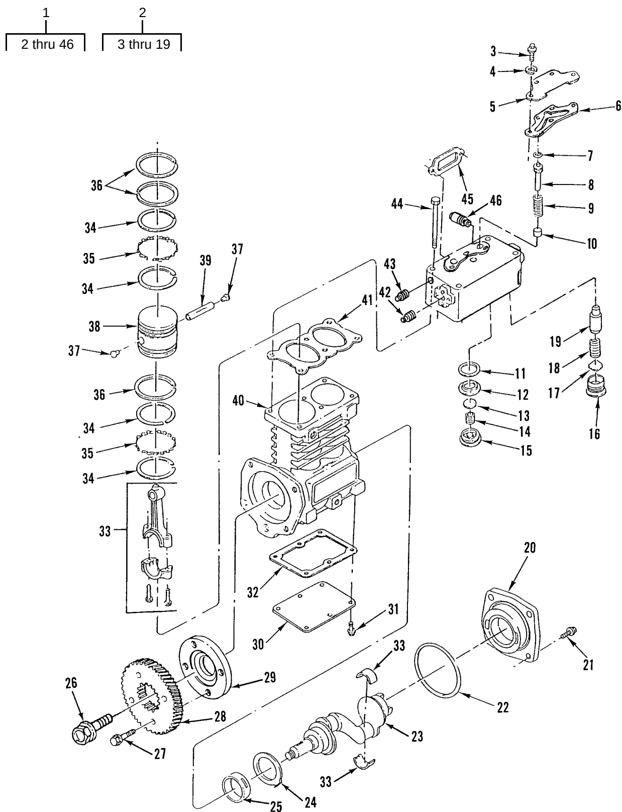
Figure 213. Air Compressor Assembly (M916A2, M917A1's)
